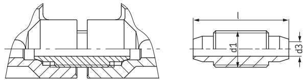
Distributor connection
